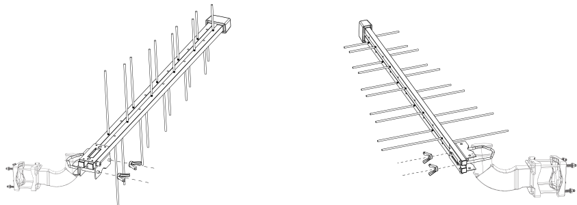
Mounted with Traditional Yagi Antenna
