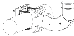
Horizontal Round Pole
