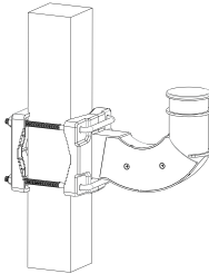
Vertical Square Pole
